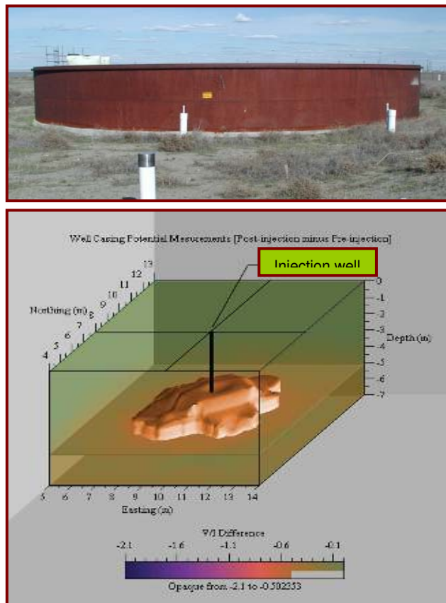
Testing of HRR-LDM in a nuclear storage tank at Hanford. Top) Picture of Mock Waste Tank. Bottom) 3D Interpretation of HRR-LDM Data
